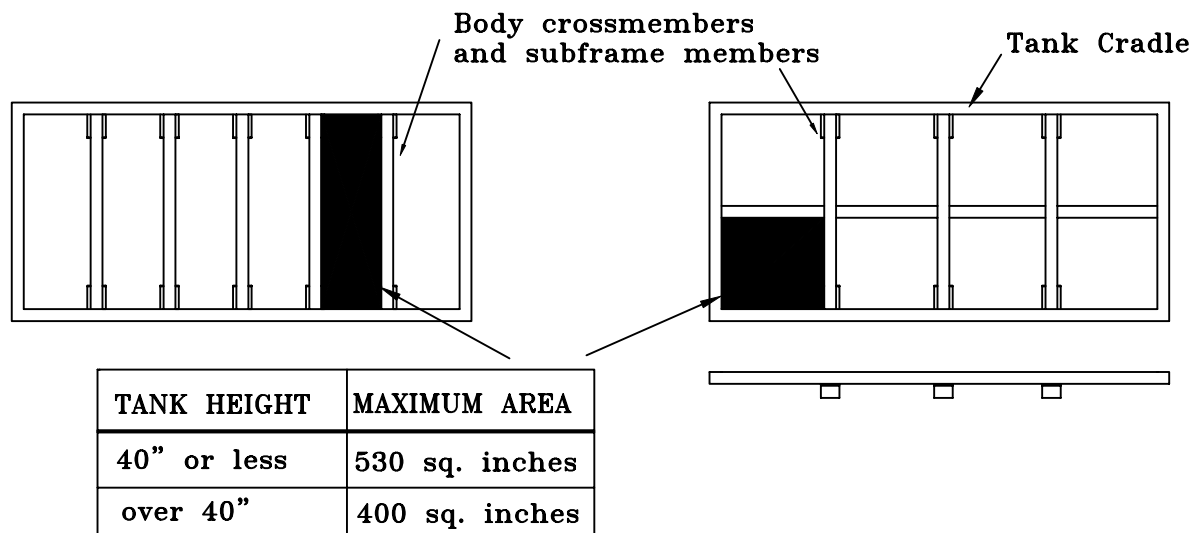
FIGURE 1: SUBFRAME SPACING
