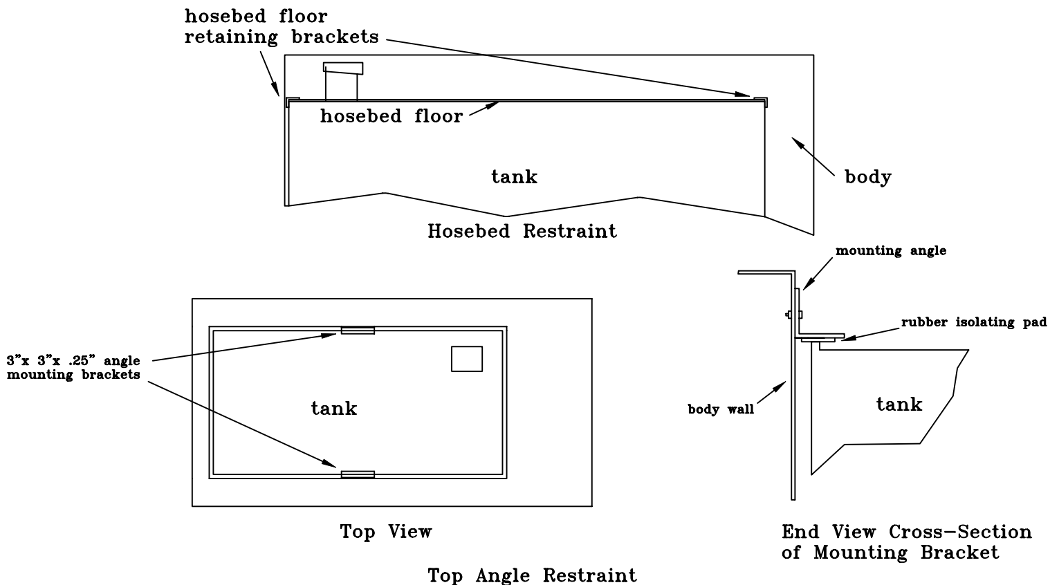
FIGURE 4: TANK HOLD DOWN
